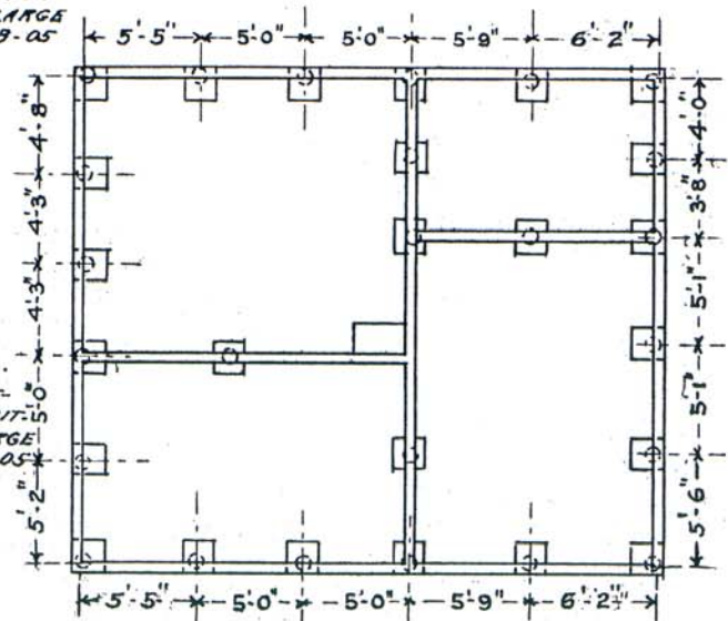
FOUNDATION PLAN
