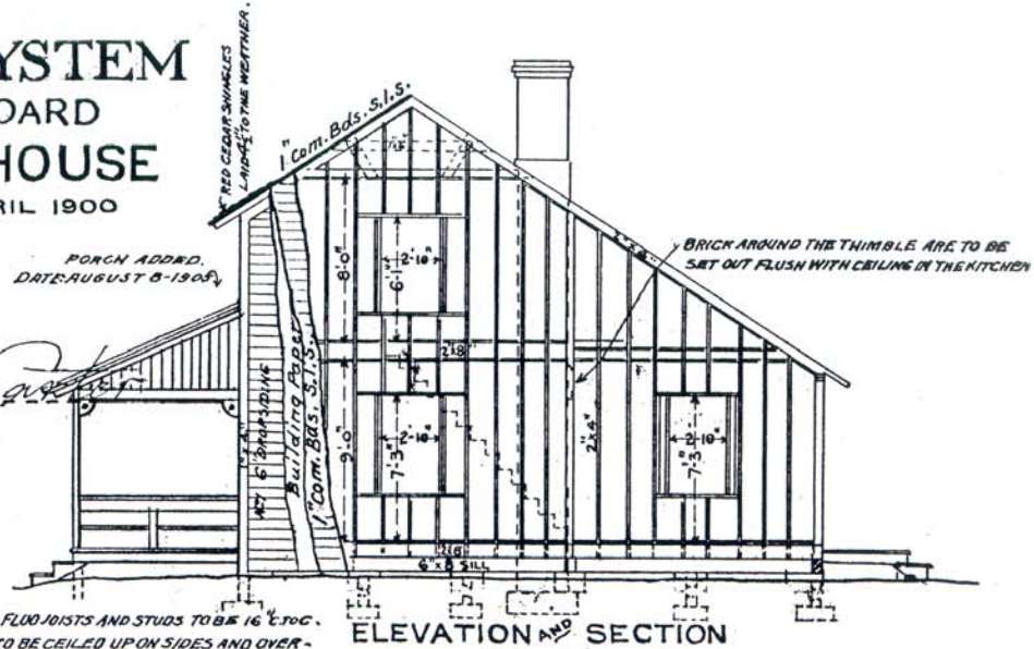
ELEVATION AND SECTION
